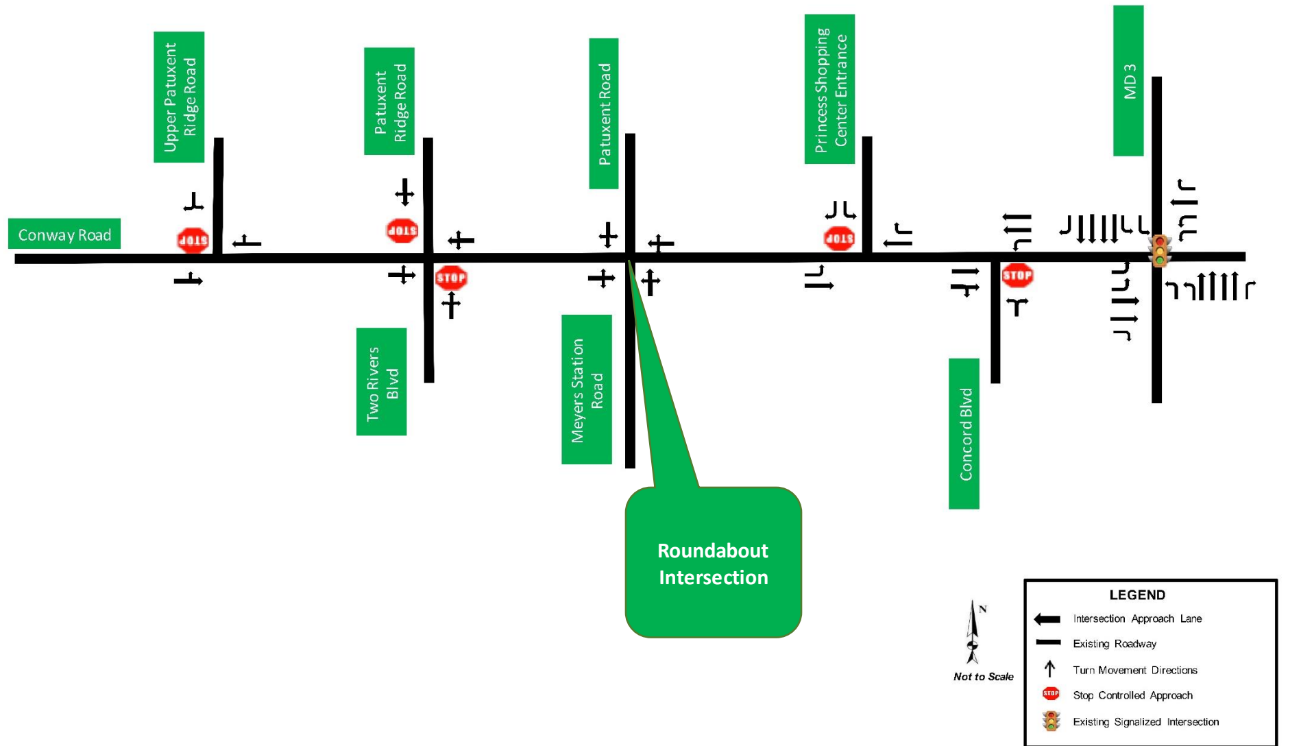
Figure 3-1: Existing Geometric Lane Configuration
