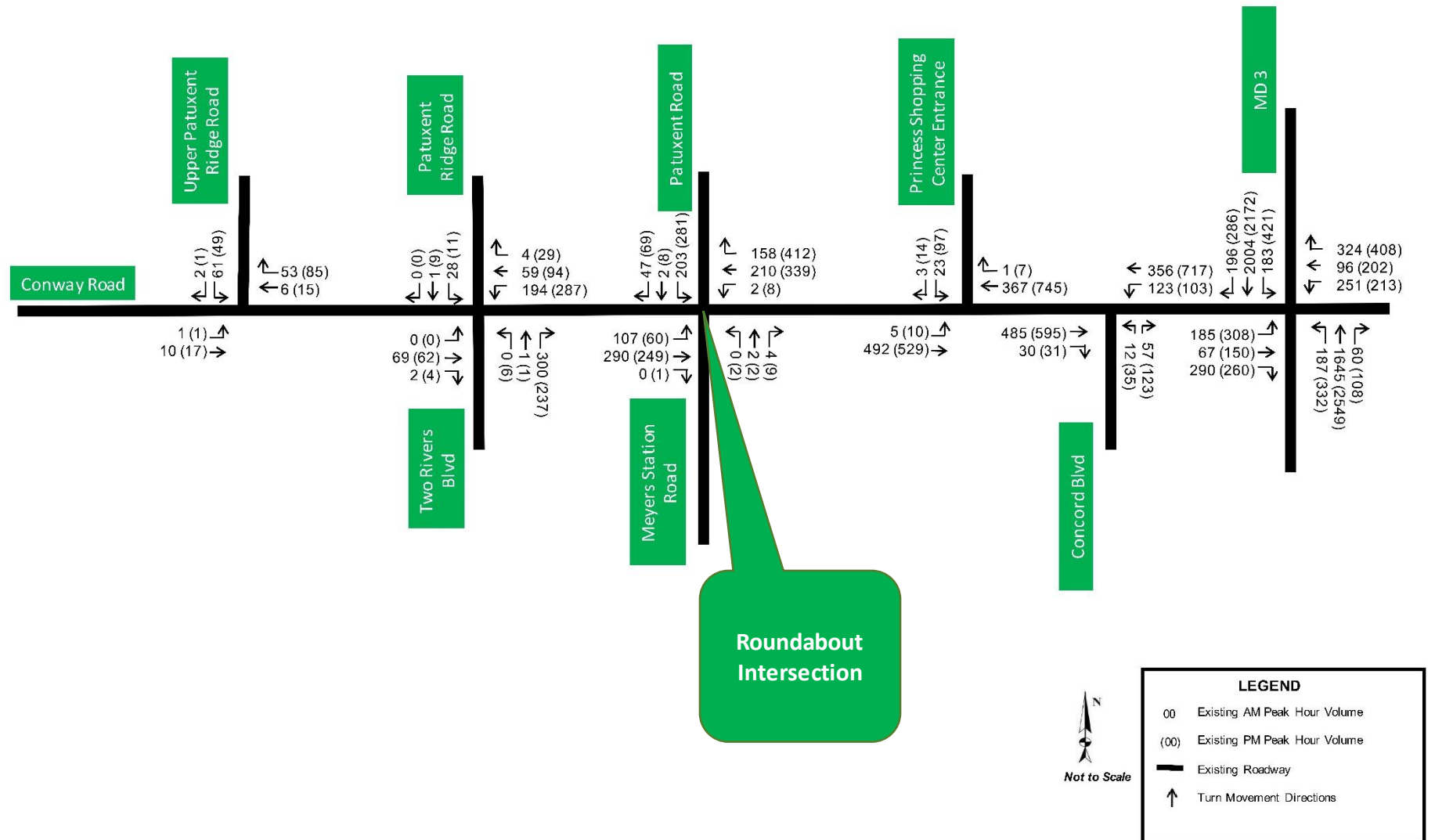
Figure 3-6: Existing Weekday Volumes
